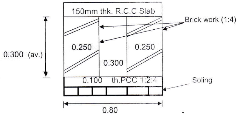
Cross section of Drain Not to Scale
